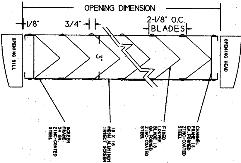
VERTICAL SECTION
